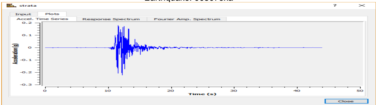
Earthquake: 005079xa
